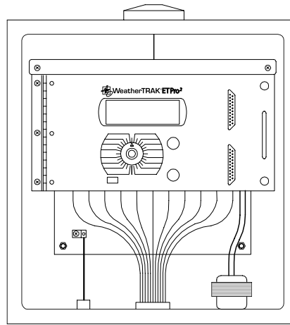
WeatherTRAK ET Pro² shown in wall mount enclosure
